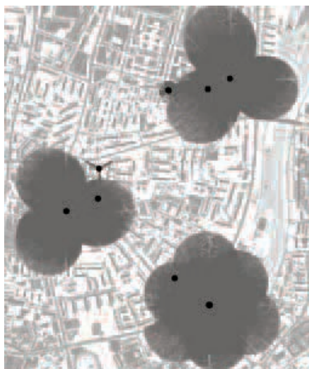
Fig. 4. Arrangement of antennas and ray propagation in experimental locality
